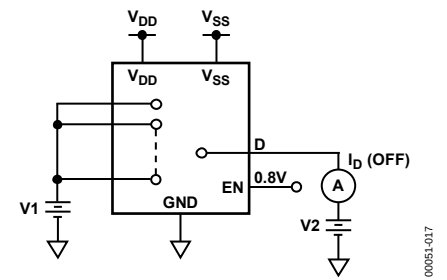
Figure 16. I_D (Off)
