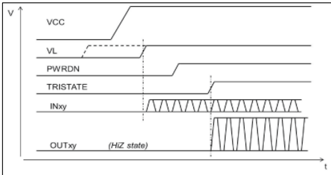
Figure 4: Power-ON sequence
