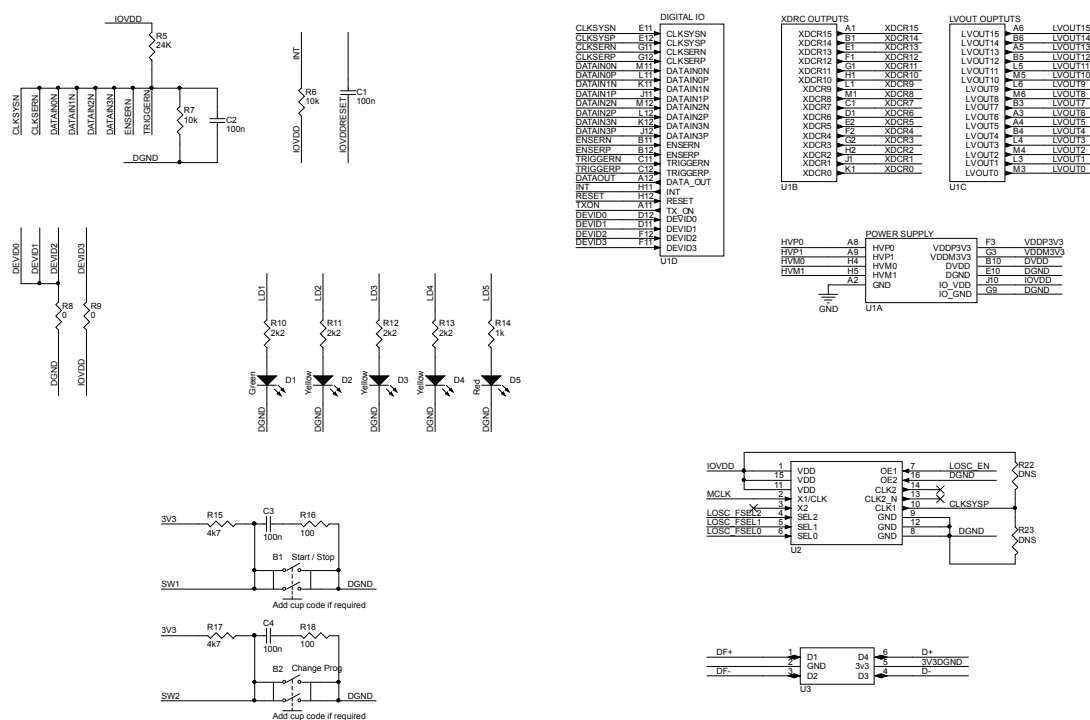
Figure 2. STEVAL-IME014V1 schematic 2
