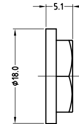
PLASTIC NUT
