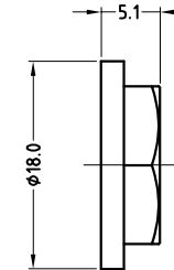
PLASTIC NUT
