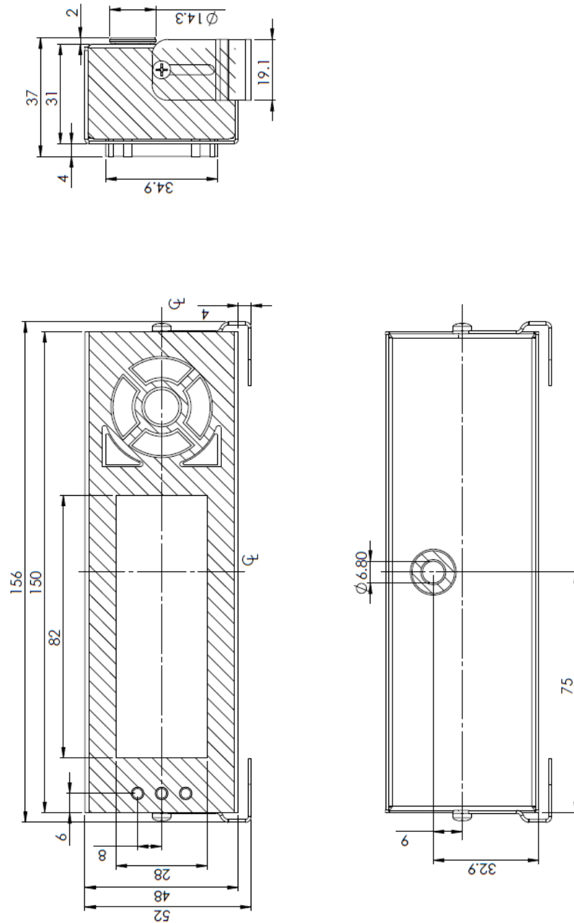
Figure 3: -MT Drawing
