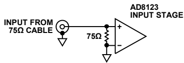
Figure 25. Terminating a 75 Ω Cable
