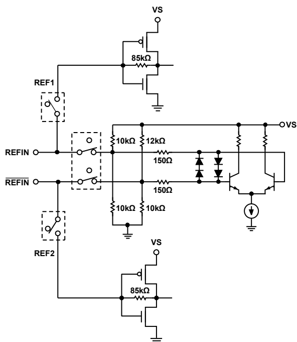
Figure 43. REF1N Equivalent Circuit for Non-XTAL Mode
