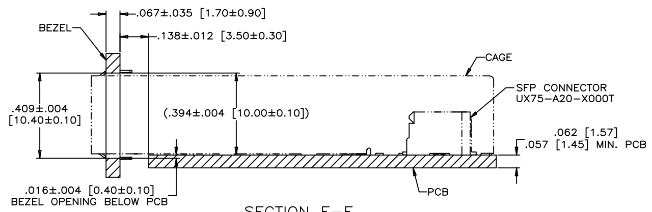
SECTION E-E
