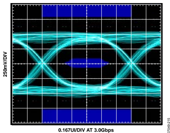
Figure 15. Tx Eye Diagram at TP2, PE = 0\text{ dB} , Data Rate = 3.0 Gbps
