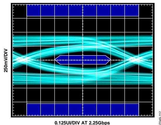
Figure 16. Tx Eye Diagram at TP3, PE = 0\text{ dB} , Data Rate = 2.25 Gbps (Cable = 6 Meters, 24 AWG)
