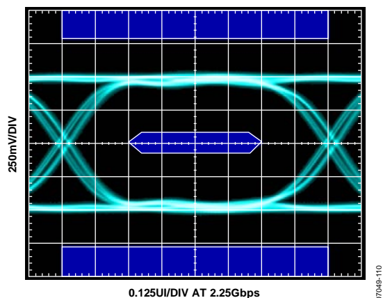
Figure 14. Tx Eye Diagram at TP2, PE = 0\text{ dB} , Data Rate = 2.25 Gbps
