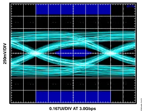
Figure 17. Tx Eye Diagram at TP3, PE = 0\text{ dB} , Data Rate = 3.0 Gbps (Cable = 6 Meters, 24 AWG)
