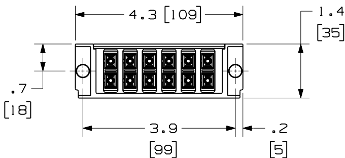
FRONT VIEW SHOWN W/O DUSTCAPS
