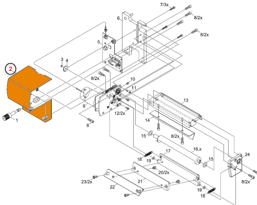
Figure 8 – T3212/T3224-PRINTER-CUTTER/PERFORTOR
