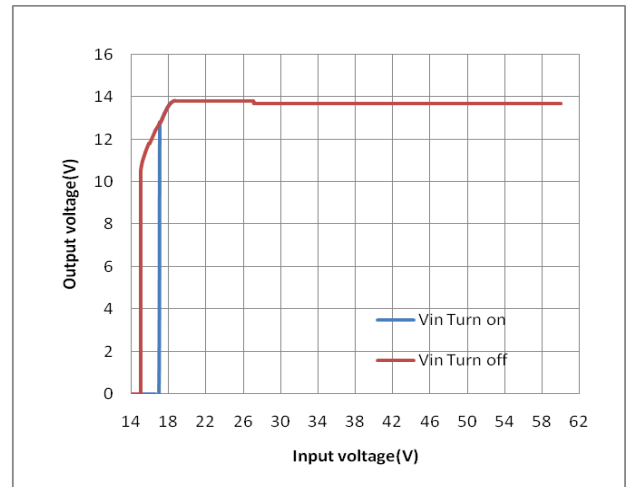
Figure 2: Output voltage vs. Input voltage @ V_{in}=18V\sim 27V, 200W ; V_{in}=27V\sim 60V, 300W
