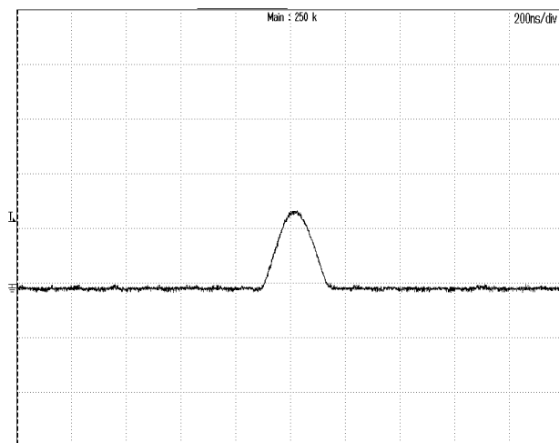
Figure 11: Inrush current @ V_{in}=48V CH1: i_{in} , 2A/div, 200ns/div Max current 2.7A, I_2t=1.24E-7 A^2S
