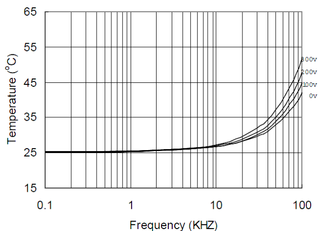
Figure 22. IR2213S vs. Frequency (IRFBC30) R gate =22Ω, V CC =15V
