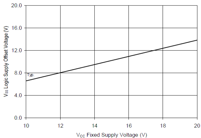
Figure 20. Maximum V SS Positive Offset vs. V CC Supply Voltage
