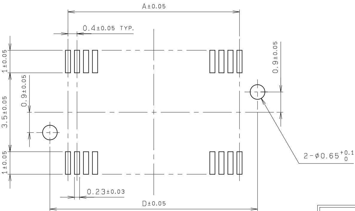
MOUNTING LAYOUT
