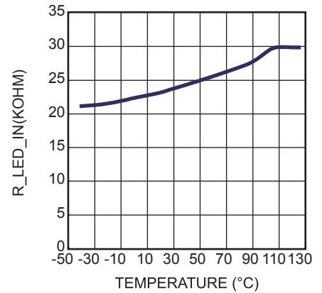
R VLED vs. Temperature
