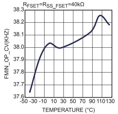
F min vs. Temperature
