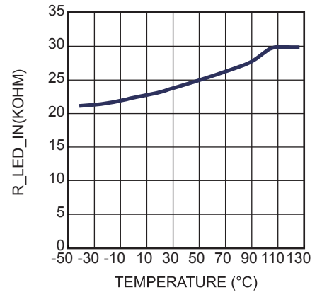
R VLED vs. Temperature
