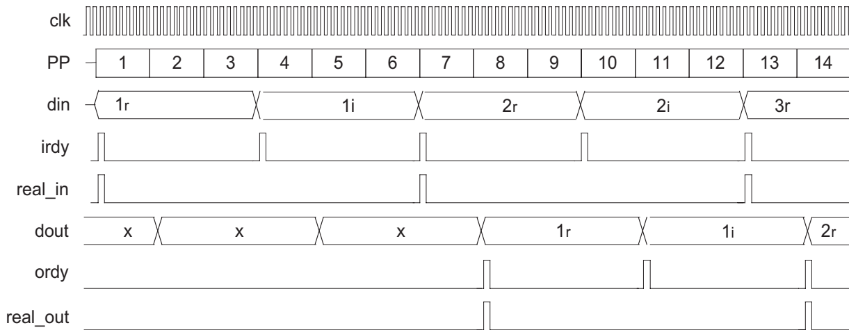
Figure 6. Timing for Multi-cycle, Complex Serial Mode
