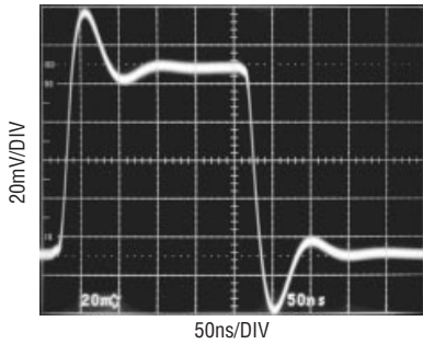
V_S = 5V A_V = 1 1215/16 G34
