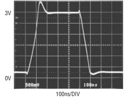
V_S = 5V A_V = -1 R_F = R_G = 1k C_F = 20pF 1215/16 G31
