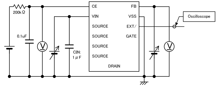
Circuit
