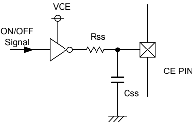
> Circuit Examle2 : CMOS logic (low current dissipation)
