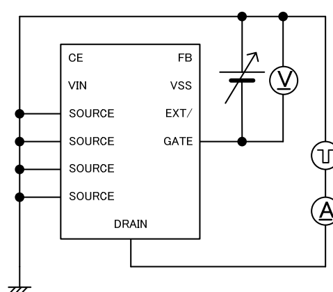
Circuit
