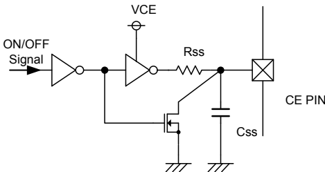
> Cicuit Examle3 : CMOS logic (low current dissipation, quick off)
