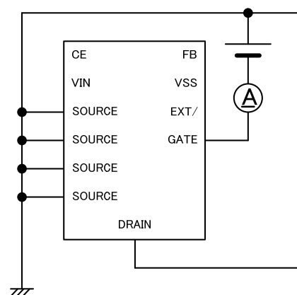
Circuit
