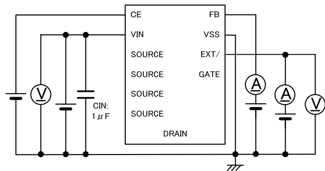
Circuit ⑤
