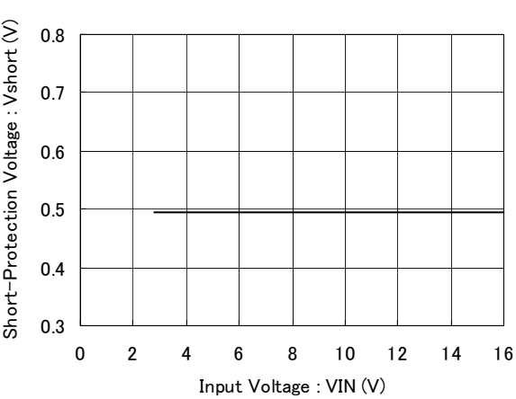
(14) Short-Circuit Protection Voltage vs. Input Voltage XCM526series
