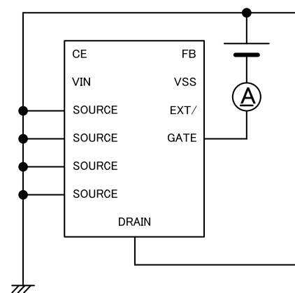
Circuit ⑨
