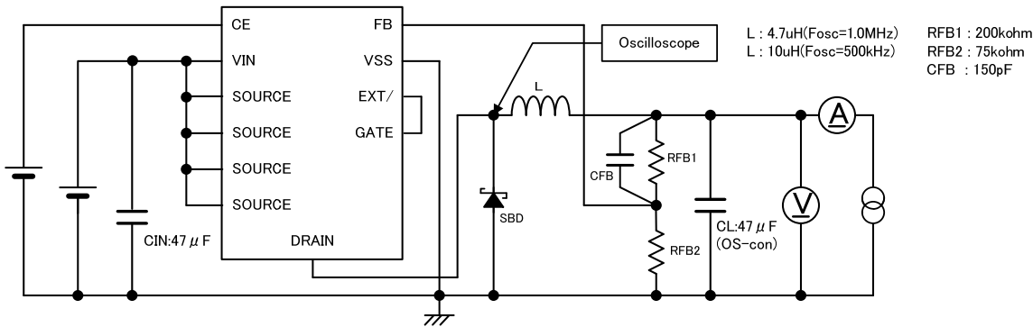
Circuit ③
