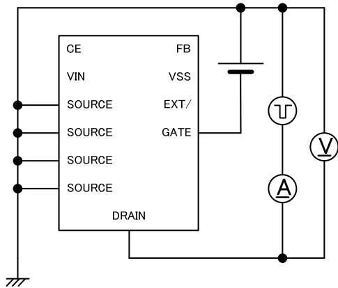
Circuit ⑫
