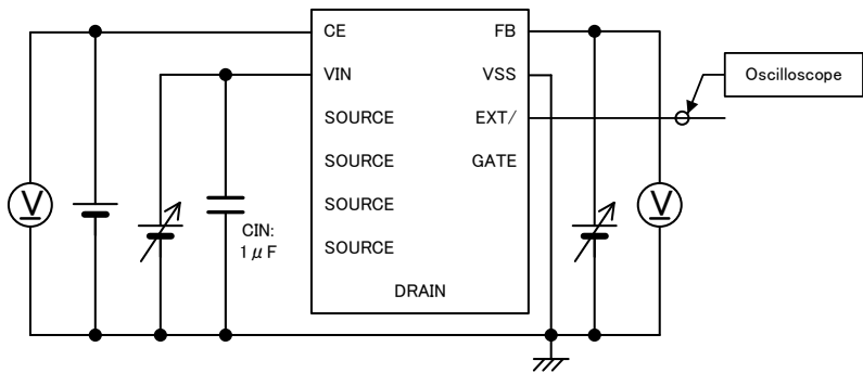
Circuit ②
