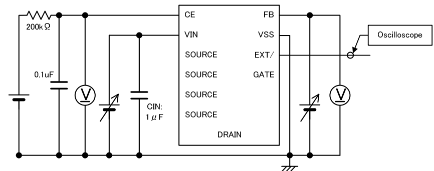
Circuit ⑤
