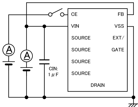
Circuit ③
