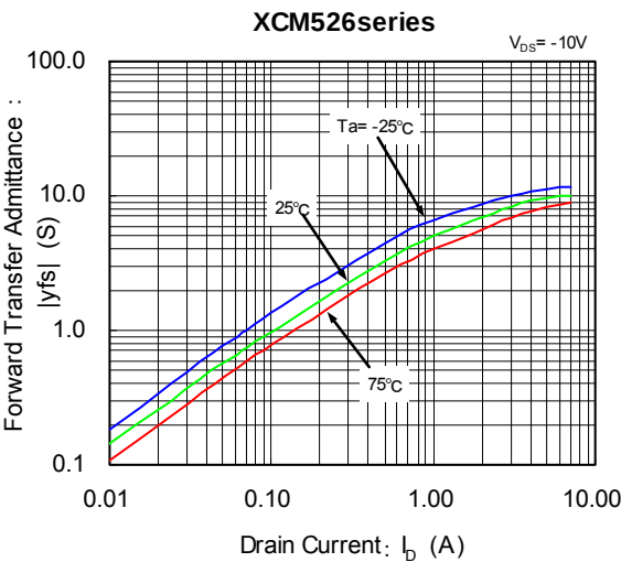
(5) Forward Transfer Admittance vs. Drain Current
