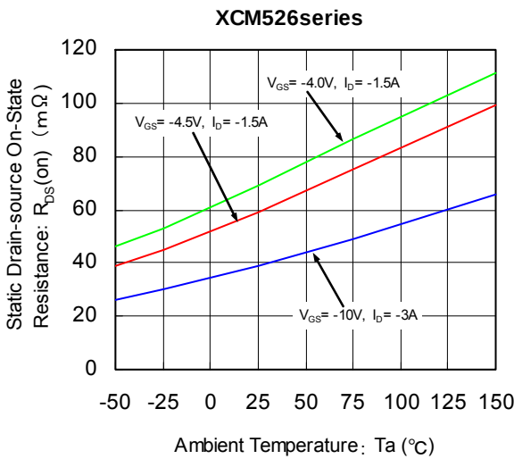
(4) Drain-Source On-State vs. Ambient Temperature
