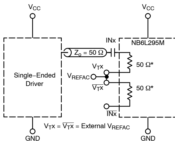
Figure 21. Capacitor-Coupled Single-Ended Interface ( V_{TX}/\overline{V_{TX}} Connected to External V_{REFAC} ; V_{REFAC} Bypassed to Ground with 0.1 μF Capacitor)
