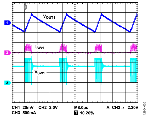
Figure 20. Typical Waveforms, V_{OUT1} = 3.3\text{ V} , Load Current = 50 mA, Auto Mode
