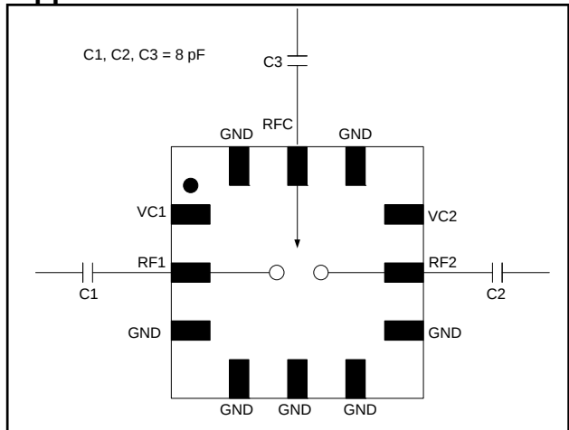
Application Schematic
