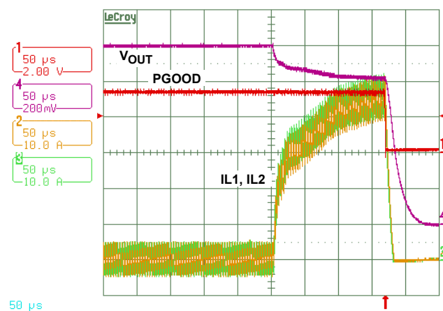
FIGURE 24. OVERCURRENT PROTECTION
