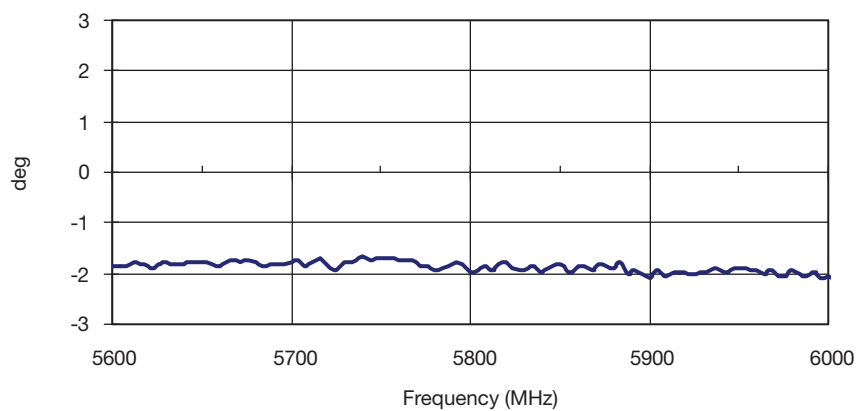
Phase Balance
