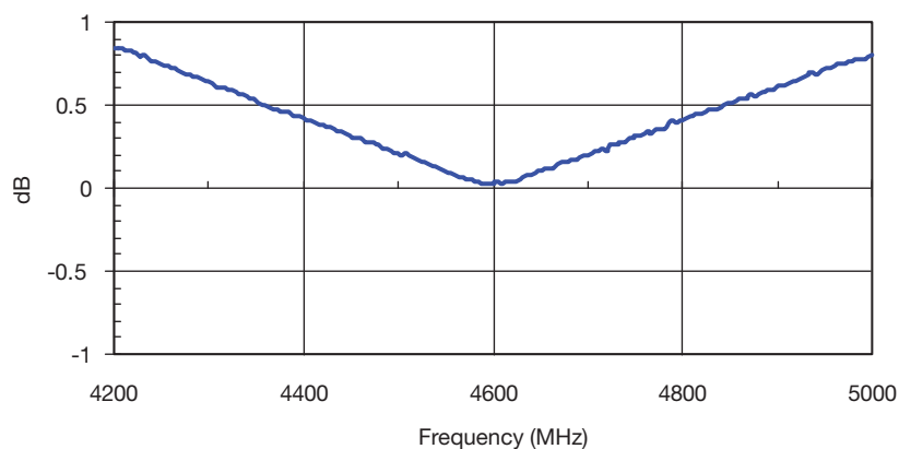
Amplitude Balance
