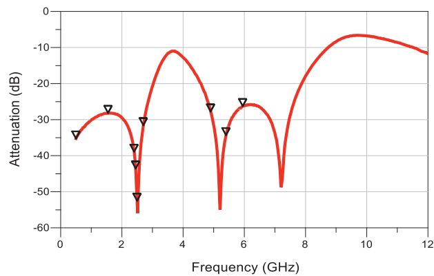
ISOLATION
