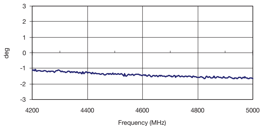
Phase Balance
