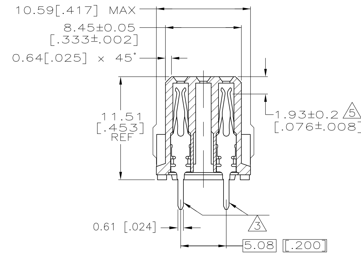
SECTION X-X
