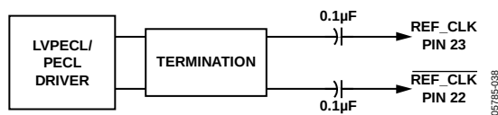
Figure 39. Typical Reference Clock Configuration for LVPECL/PECL Source
