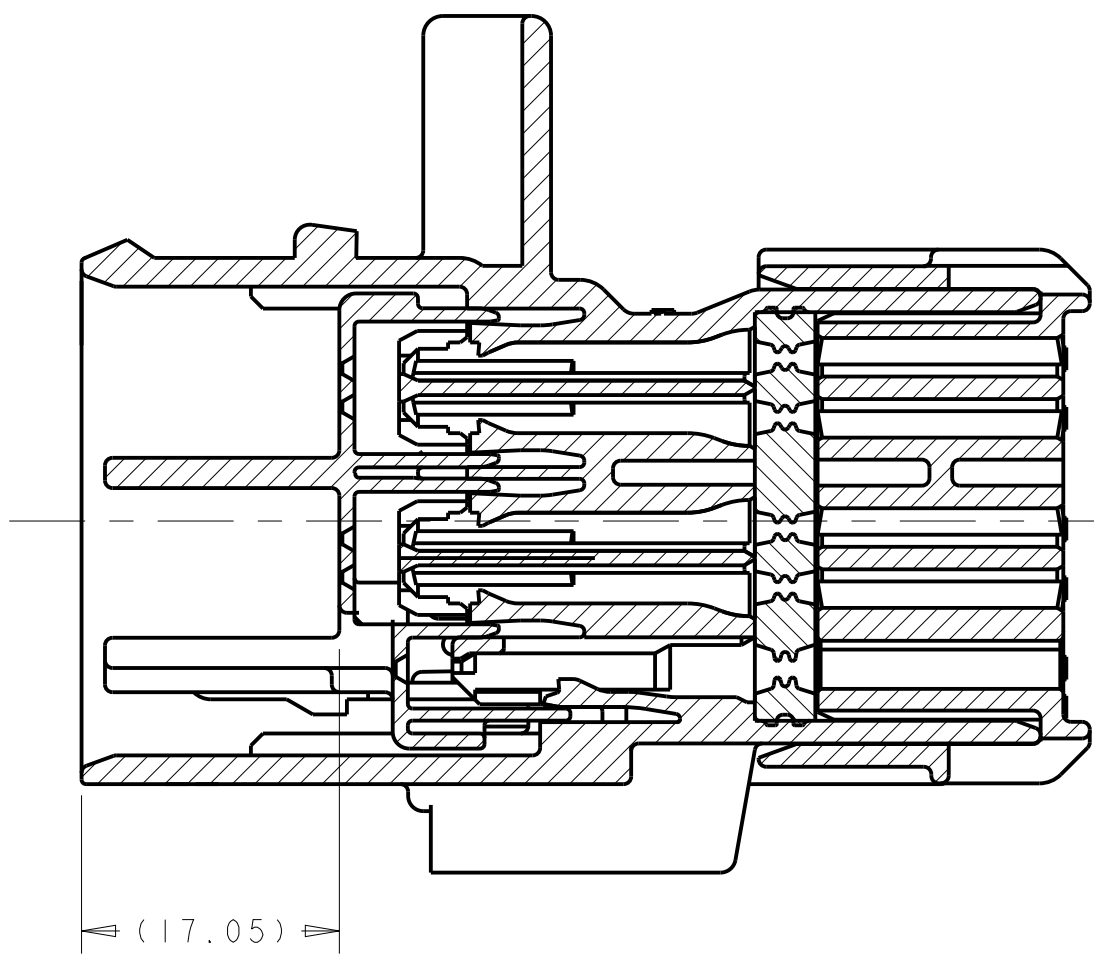
SECTION A-A TPA SHOWN IN ITS SHIPPING POSITION FROM THE HARNESS ASSEMBLY PLANT.
