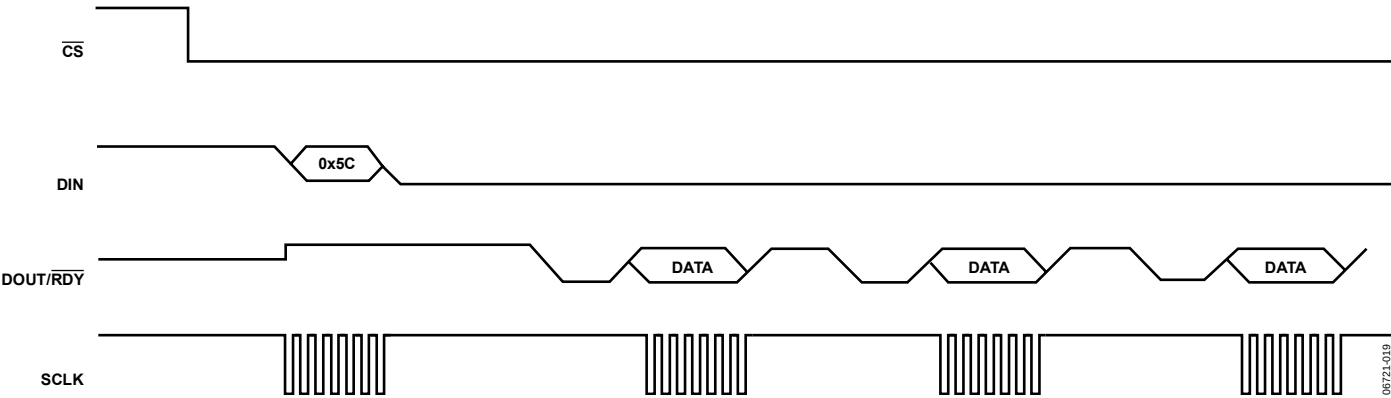
Figure 19. Continuous Read
