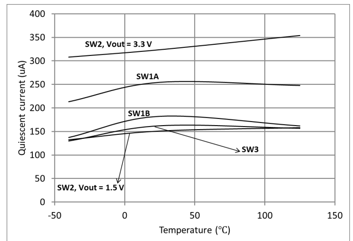
Figure 23. Quiescent current - buck regulators in APS mode
