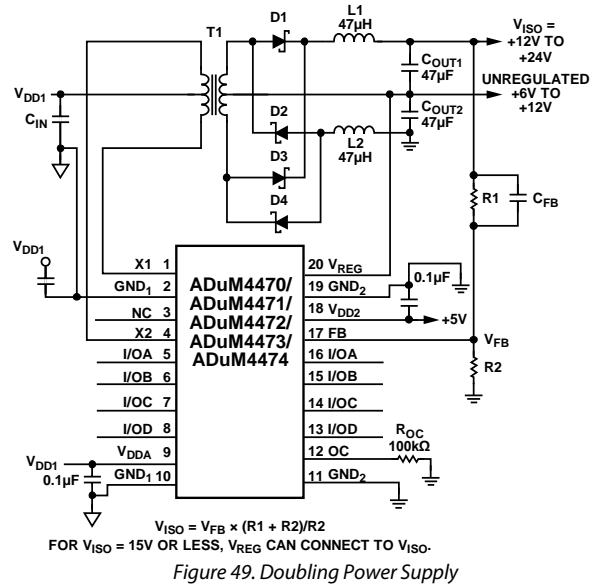
Figure 49. Doubling Power Supply
