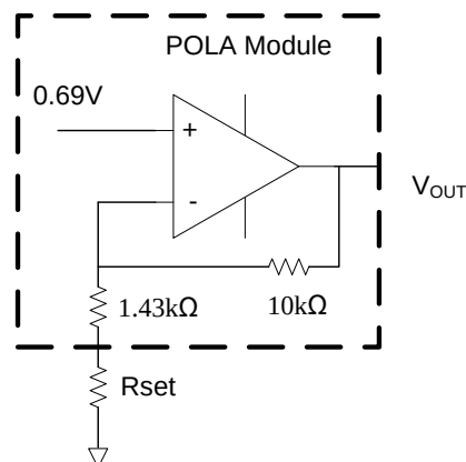
Figure 11. Output Voltage Setting on POLA Module
