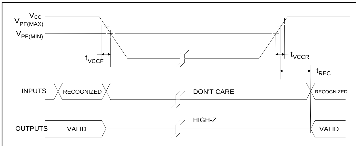
Figure 1. Power-Up/Down Timing
