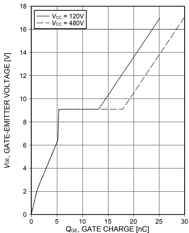
Figure 17. Typical gate charge ( I_C=4A )
