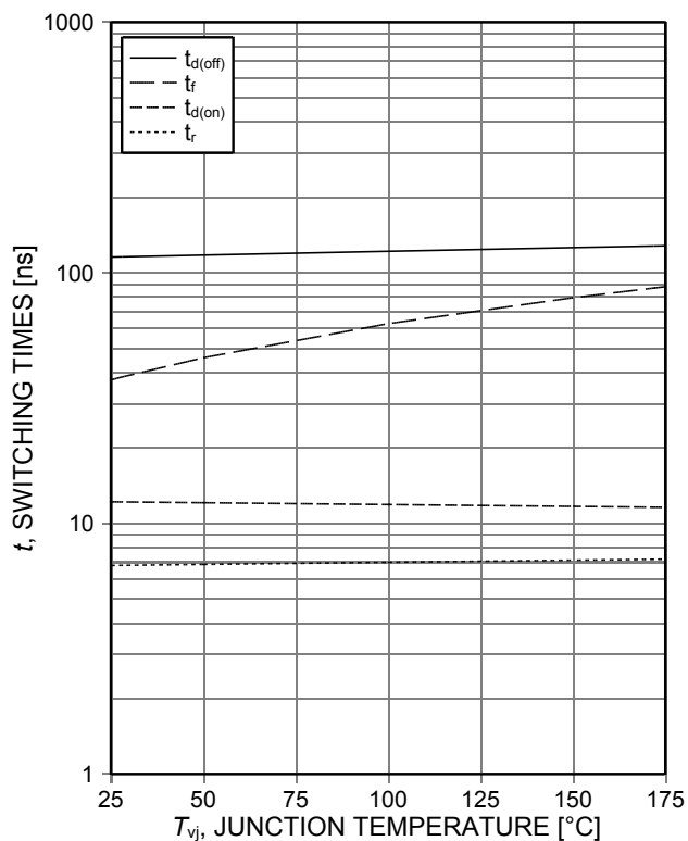
Figure 11. Typical switching times as a function of junction temperature (inductive load, V_{CE}=400\text{V} , V_{GE}=15/0\text{V} , I_C=4\text{A} , r_G=43\Omega , Dynamic test circuit in Figure E)
