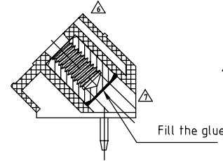
SECTION P-P
