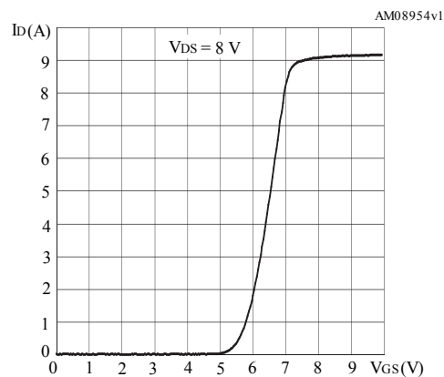
Figure 6. Transfer characteristics
