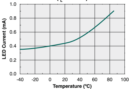
Typical I F for Switch Operation vs. Temperature (I L =120mA)
