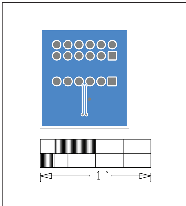
MAX31875 EV Kit—Bottom
