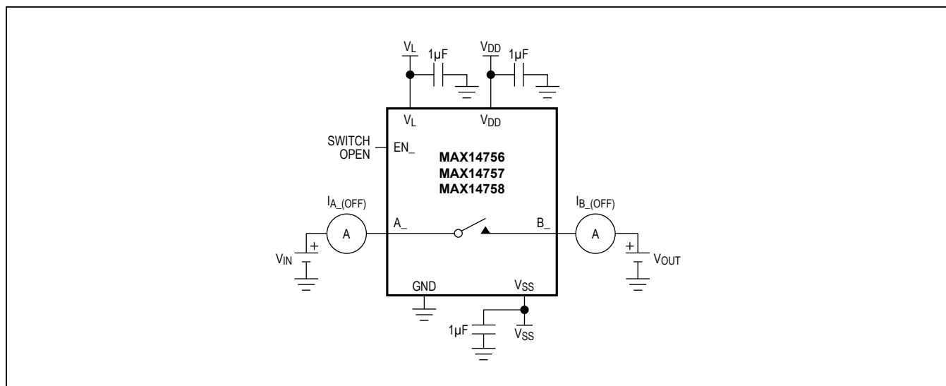
Figure 3. Off-Leakage Current
