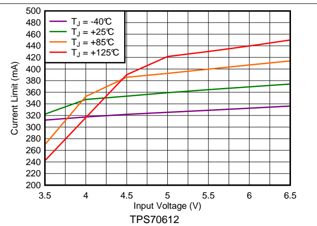
Figure 6. 1.2-V Current Limit vs V_{IN} and Temperature
