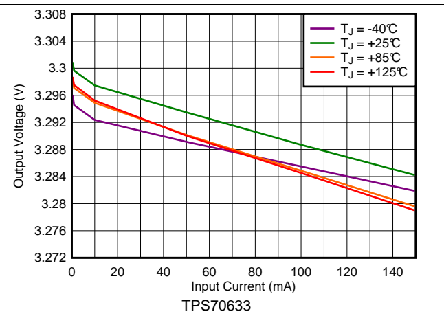
Figure 4. 3.3-V Load Regulation vs I_{OUT} and Temperature
