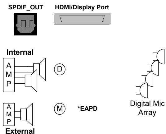
Figure 24. Port Configurations
