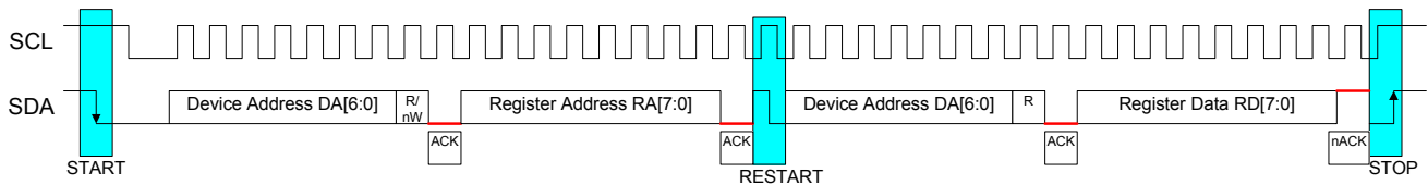
Figure 19. Read Cycle
