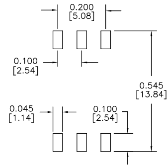
Recommended Solder Pad Dimensions
