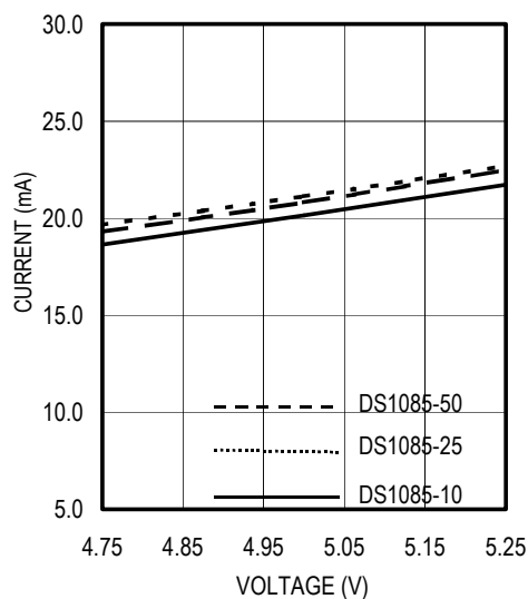
SUPPLY CURRENT vs. VOLTAGE
