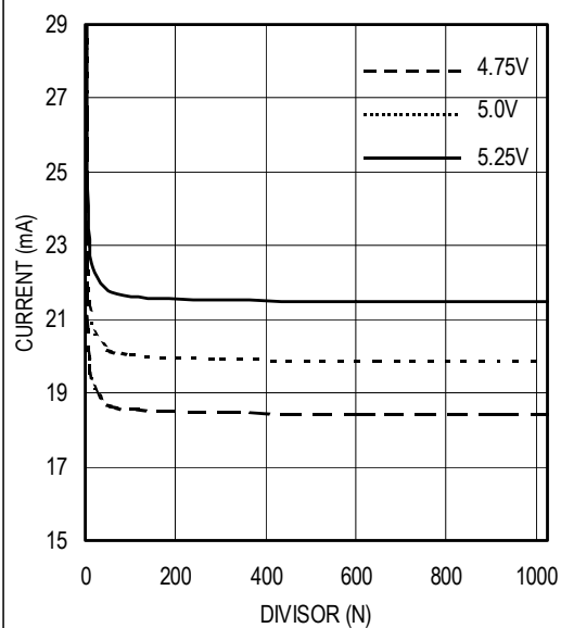
SUPPLY CURRENT vs. DIVISOR
