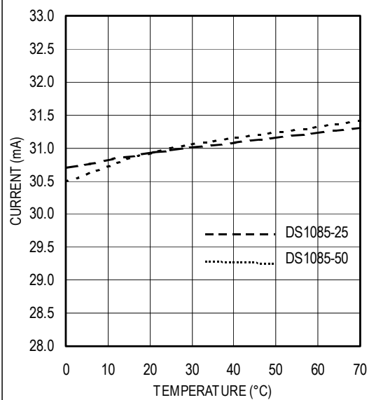
SUPPLY CURRENT vs. TEMPERATURE
