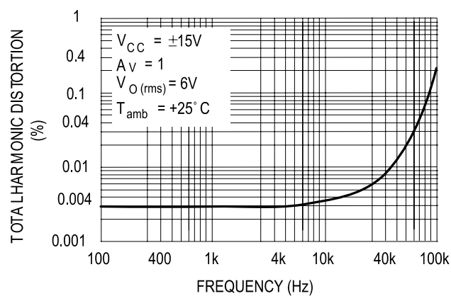
Figure 19: Total harmonic distortion versus frequency
