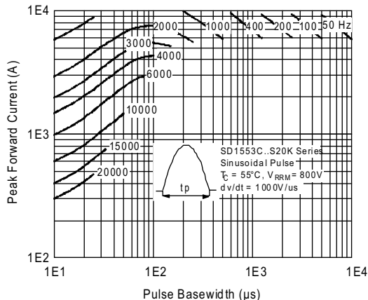
Fig. 29 - Frequency Characteristics
