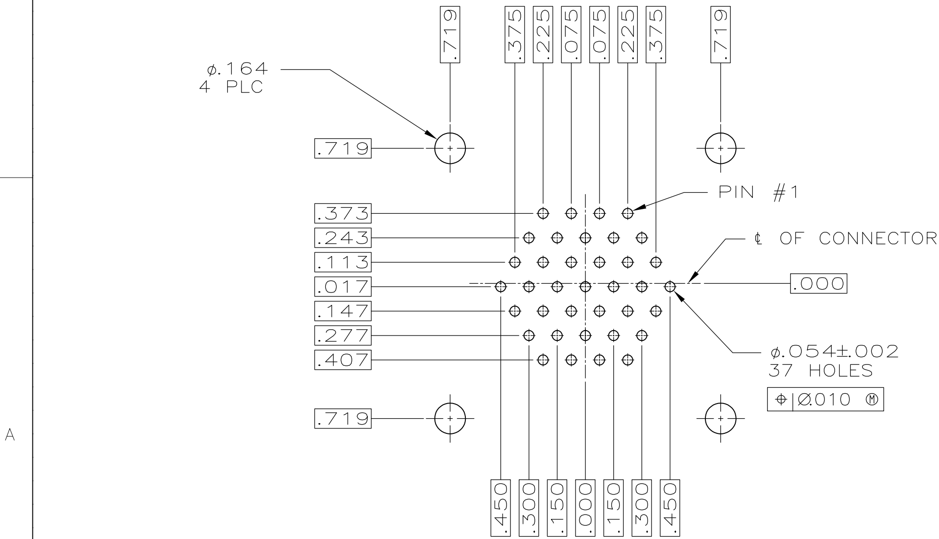
RECOMMENDED P.C. BOARD LAYOUT
