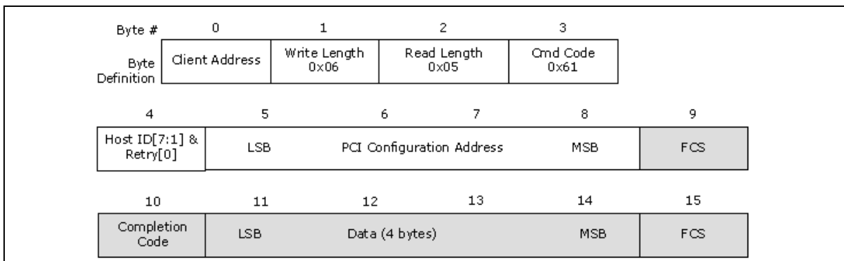
Figure 2-45. RdPCICfg()
